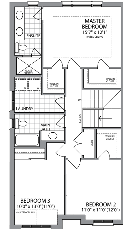
UPPER LEVEL - ELEV. B
