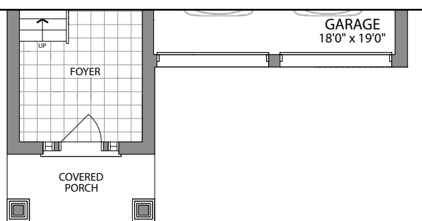
PARTIAL MAIN LEVEL ELEV. C
