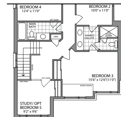
PARTIAL UPPER LEVEL ALT. 5 BDRM OR DEN ELEV. C
