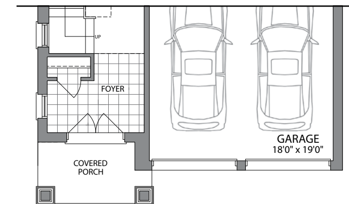
PARTIAL MAIN LEVEL ELEV. B
