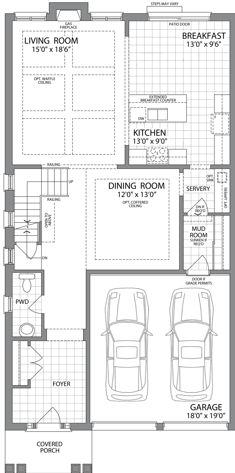
MAIN LEVEL - ELEV. A
