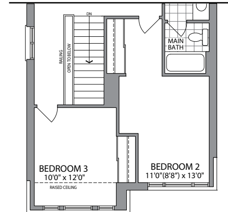
PART. UPPER LEVEL ELEV. C
