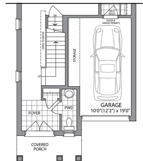
PART. MAIN LEVEL ELEV. B
