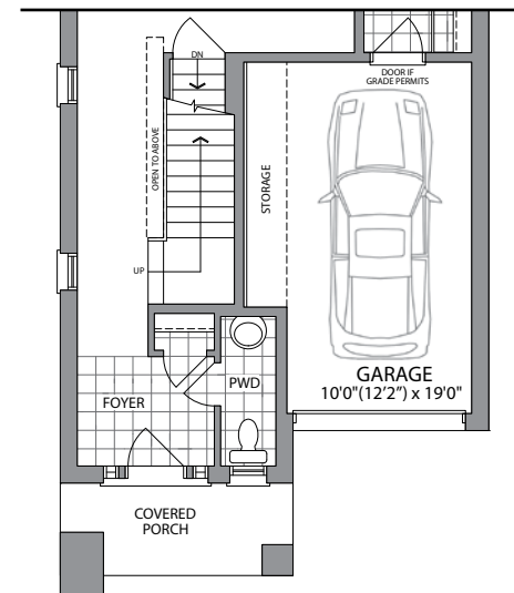
PART. MAIN LEVEL ELEV. C
